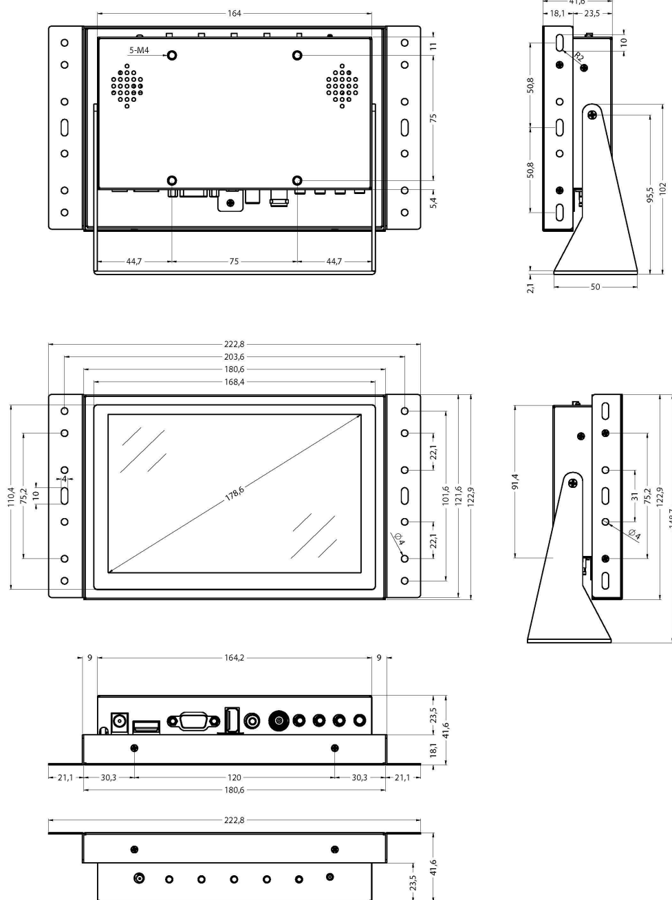
7TS7M
